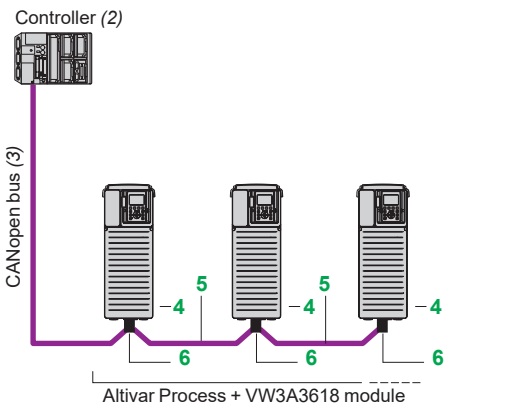
Example of connection to the CANopen bus via SUB-D connector
